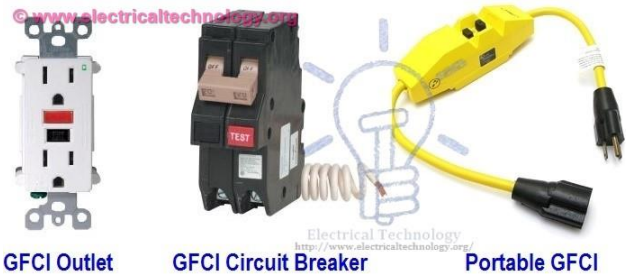
GFCI Outlet
