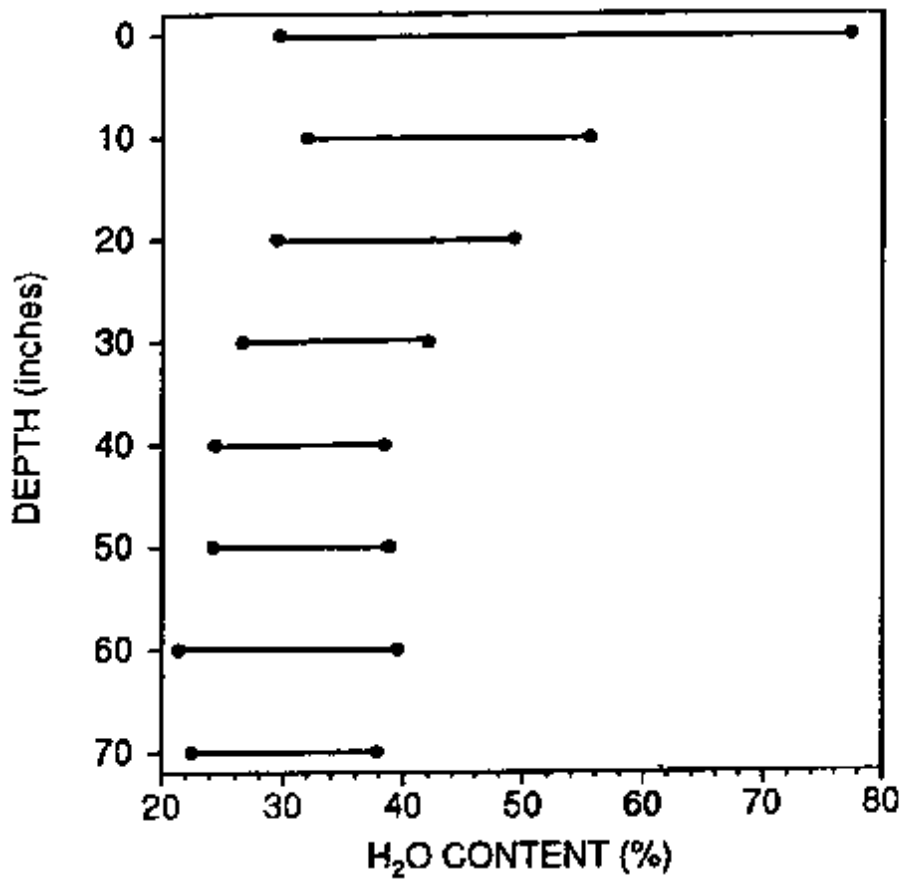
Figure 13. Average soil moisture content range, 1991-1995, for sites 1, 3, and 4.
