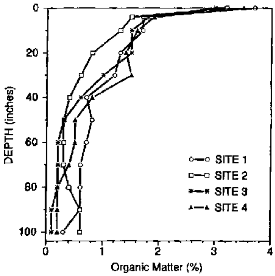
Figure 6. Soil organic matter distribution of representative Sharkey soils.
