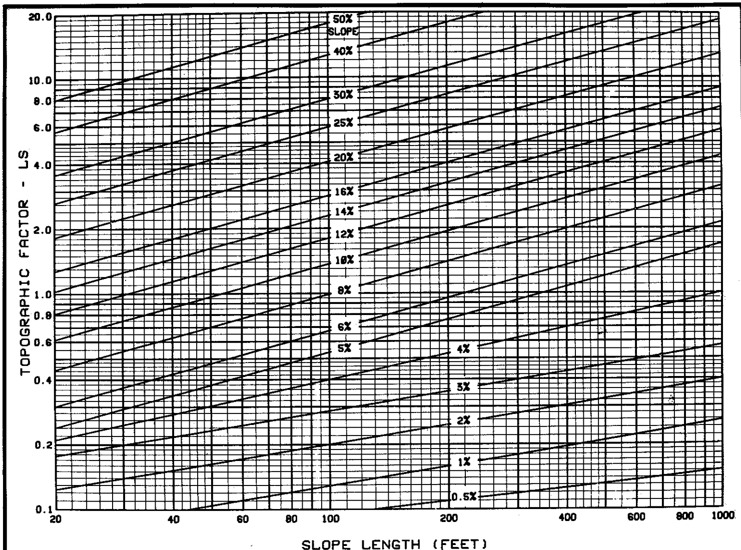
Figure 3. A nomograph which simplifies estimation of the length-slope factor.
