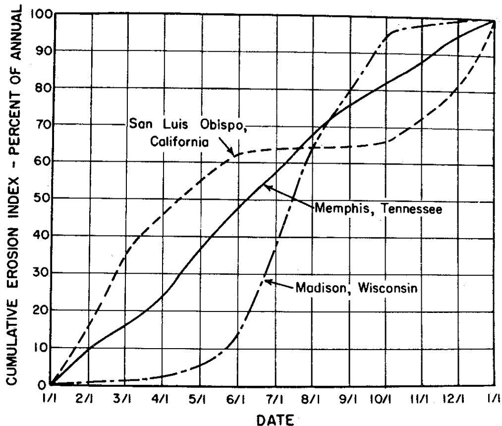
Figure 4. Cumulative erosivity index reveals non-uniform rainfall patterns.
