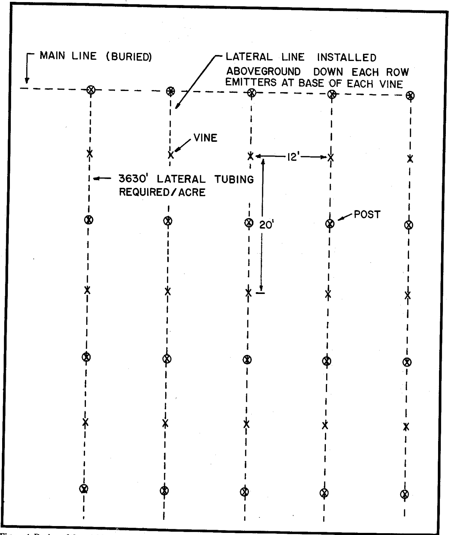
Figure 4. Design of the trickle irrigation system that requires 3630' of lateral tubing per acre.
