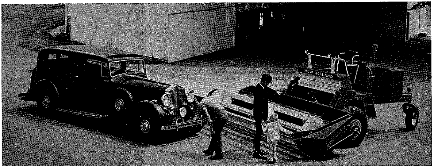
Figure 2. A self-propelled harvesting machine (right) for cutting, conditioning and wind-rowing alfalfa.
